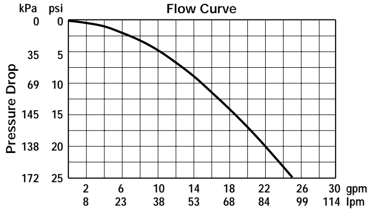
Flow Chart
